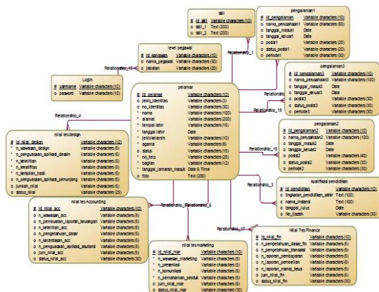
Gambar 2. Conceptual Data Model (CDM)
