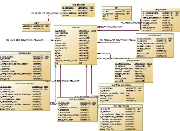
Gambar 3. Physical Data Model (PDM)
